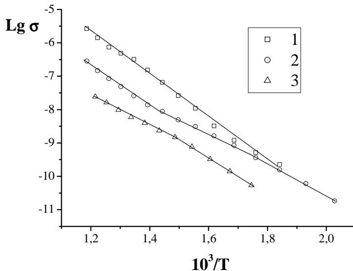
Рис. 3. Залежність \text{Lg}(\sigma) - 1000/t (К): 1 – \text{LiIn}_{0,6}\text{Fe}_{0,4}\text{P}_2\text{O}_7 ; 2 – \text{NaIn}_{0,58}\text{Fe}_{0,42}\text{P}_2\text{O}_7 ; 3 – \text{KIn}_{0,8}\text{Fe}_{0,2}\text{P}_2\text{O}_7
