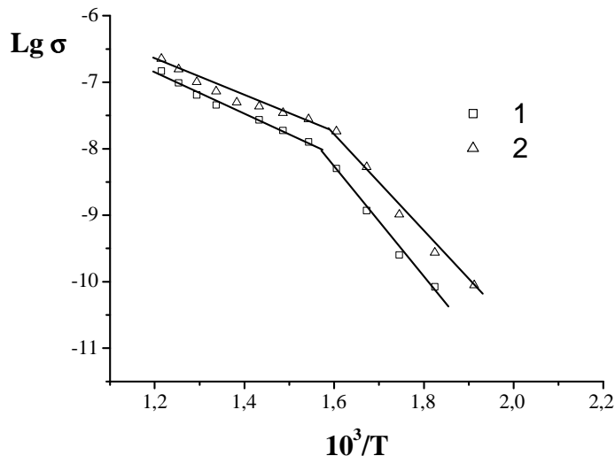
Рис. 4. Залежність \text{Lg}(\sigma) - 1000/t (К): 1 – \text{Na}_7(\text{In}_{0,82}\text{Cr}_{0,18}\text{P}_2\text{O}_7)_4\text{PO}_4 ; 2 – \text{Na}_7(\text{In}_{0,98}\text{Mn}_{0,02}\text{P}_2\text{O}_7)_4\text{PO}_4
